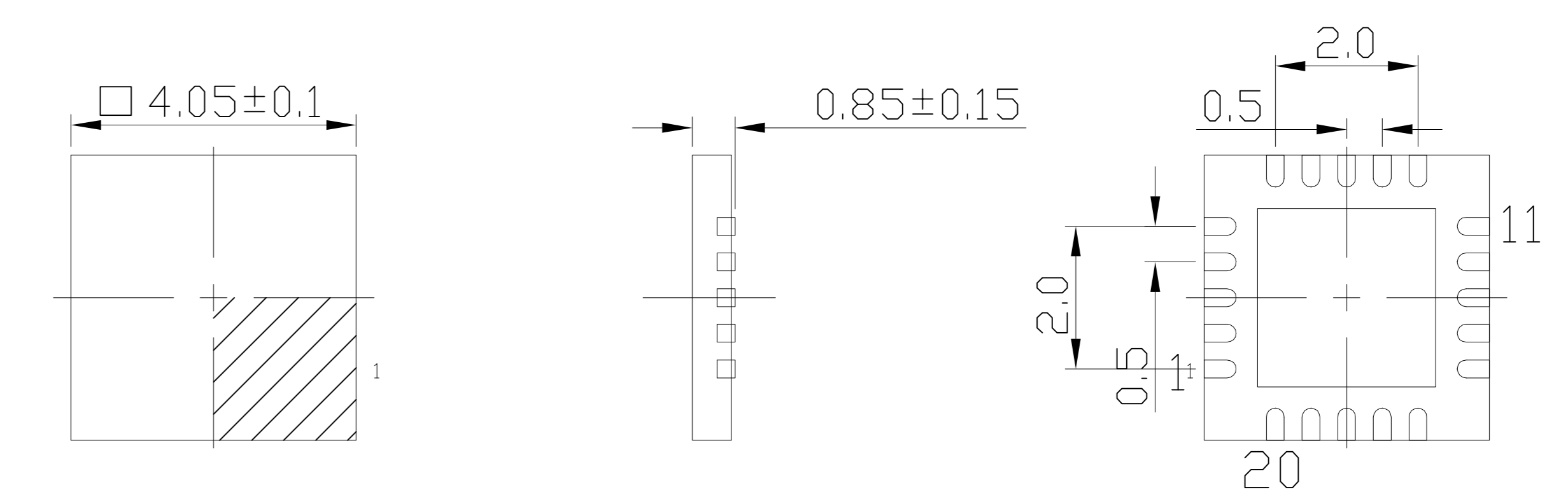
TOP VIEW
