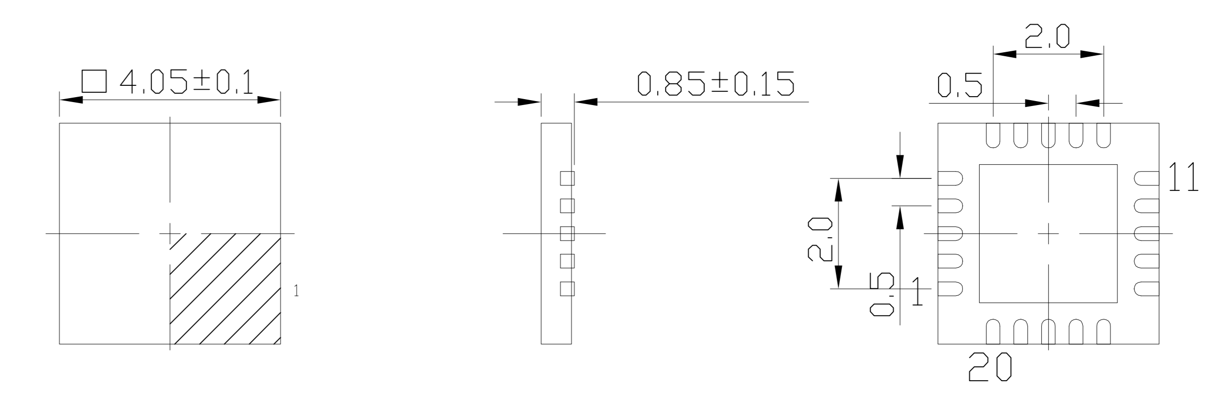
TOP VIEW
